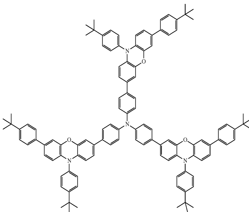
Compound 2
